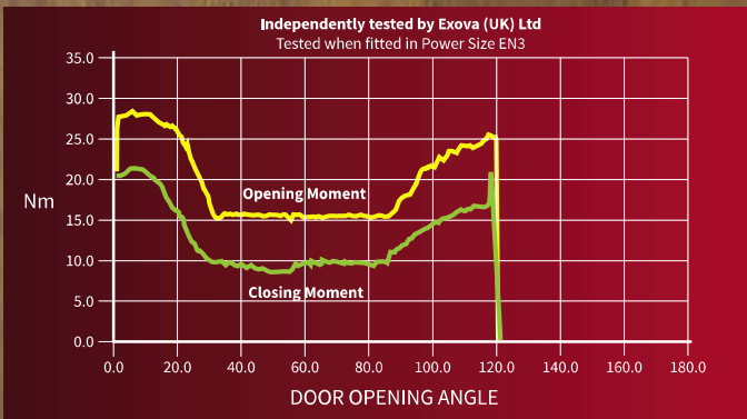
Power curve
